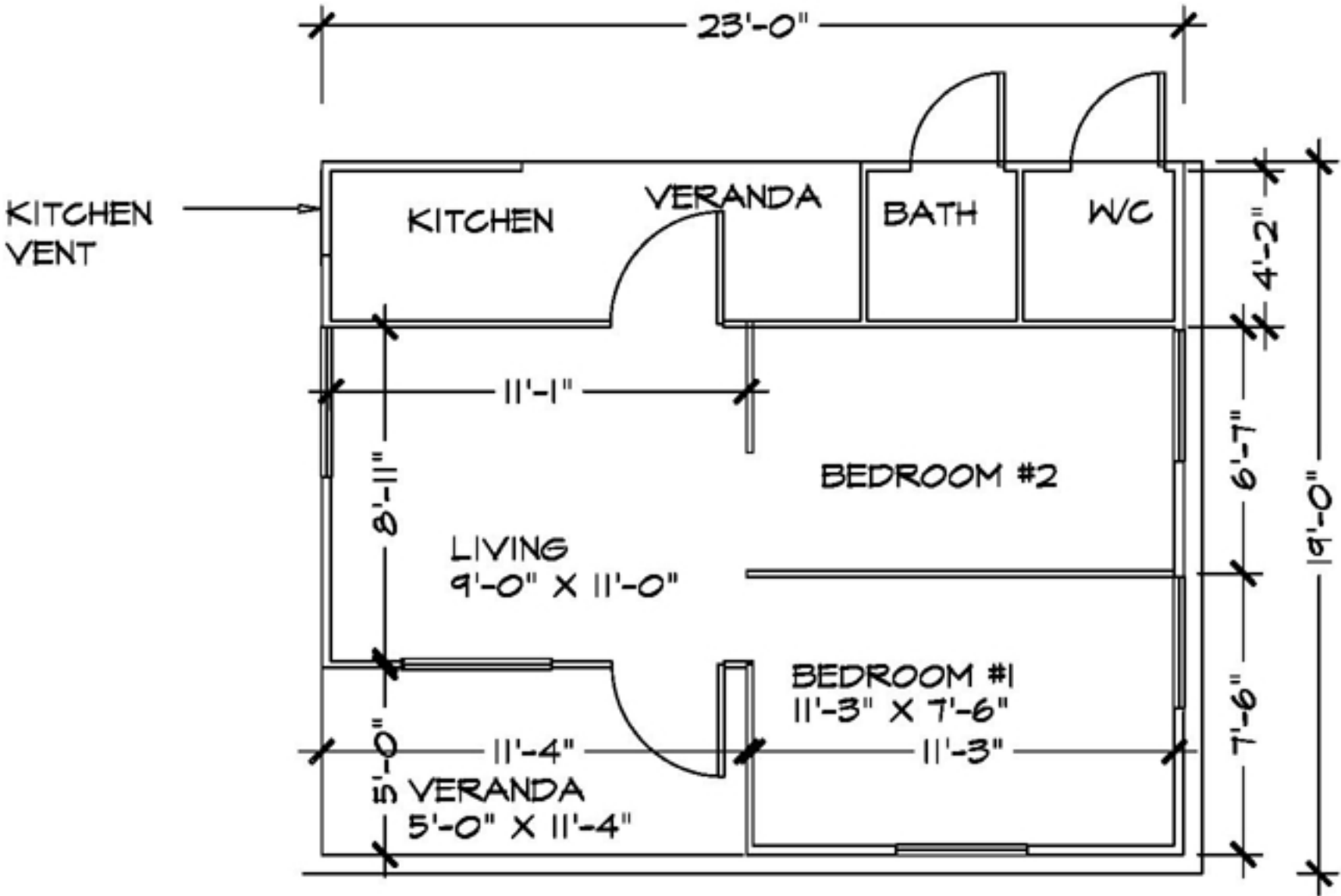
FLOORPLAN
